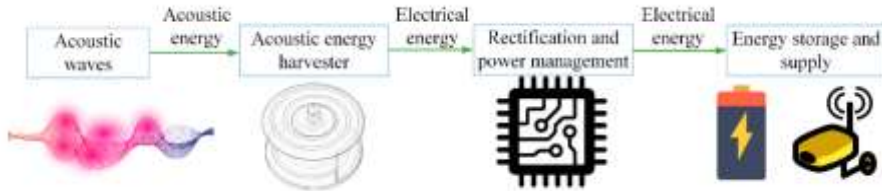
Figure 11.4. Schematic diagram of an acoustic energy-harvesting (AEH) system (Yuan et al., 2019)
