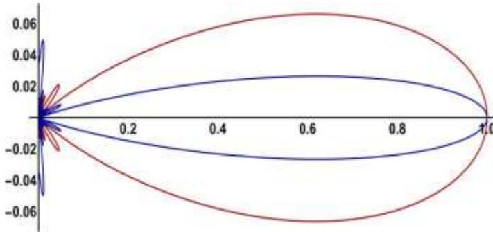
Figure 11. 2. Polar plot of line system sound, contains from 10 loudspeakers at the 60 cm distance, for 2000 Hz (red line) and 5000 Hz (blu line) (Popović & Ilić, 2018)
