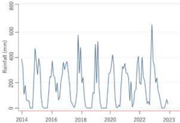
Figure 6. 1. Rainfall time series from January 2014 to December 2023
